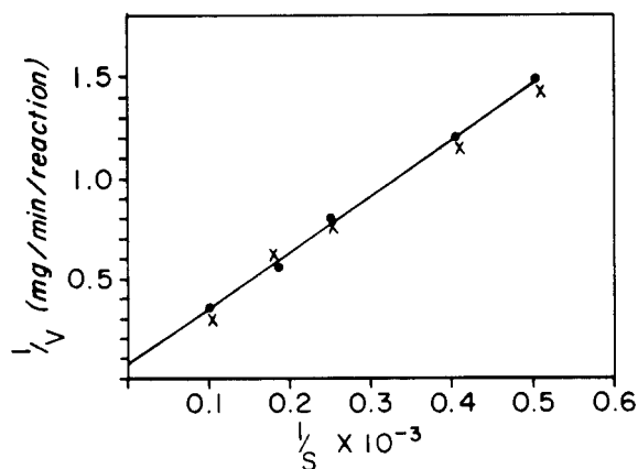
FIG. 10.—The reciprocal plot of fatty acid released by action of proteins I (●-●) and II (X-X) against substrate (lecithin) concentration. The details of these experiments are described in the text. Reaction time, 15 minutes.
